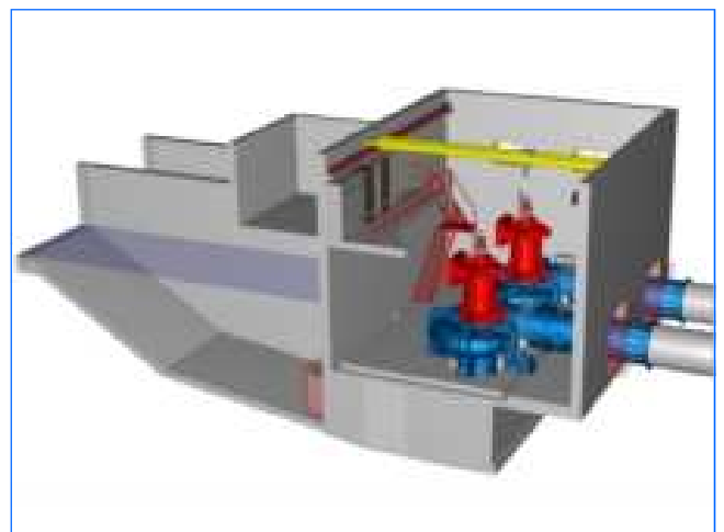
CAD Einbauplan CAD assembly drawing
