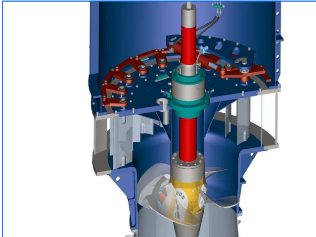
Kaplanturbine 3D Kaplan turbine 3D
