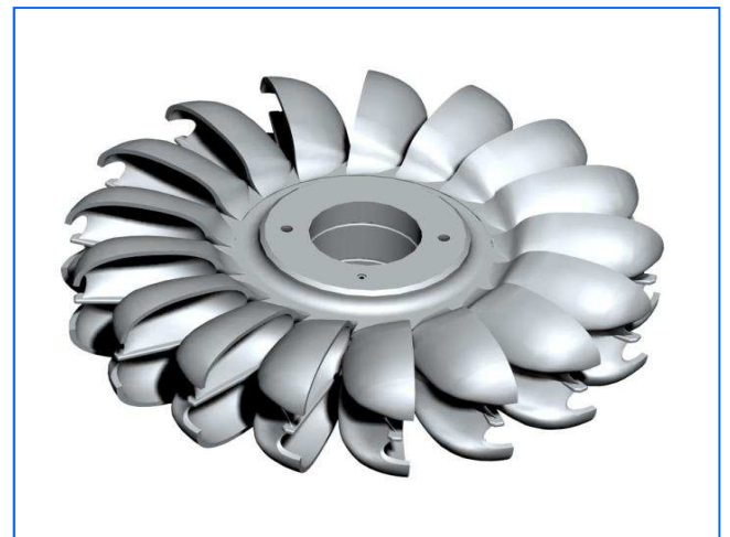
CAD-Modell Pelton Laufrad 3D CAD model Pelton runner 3D
